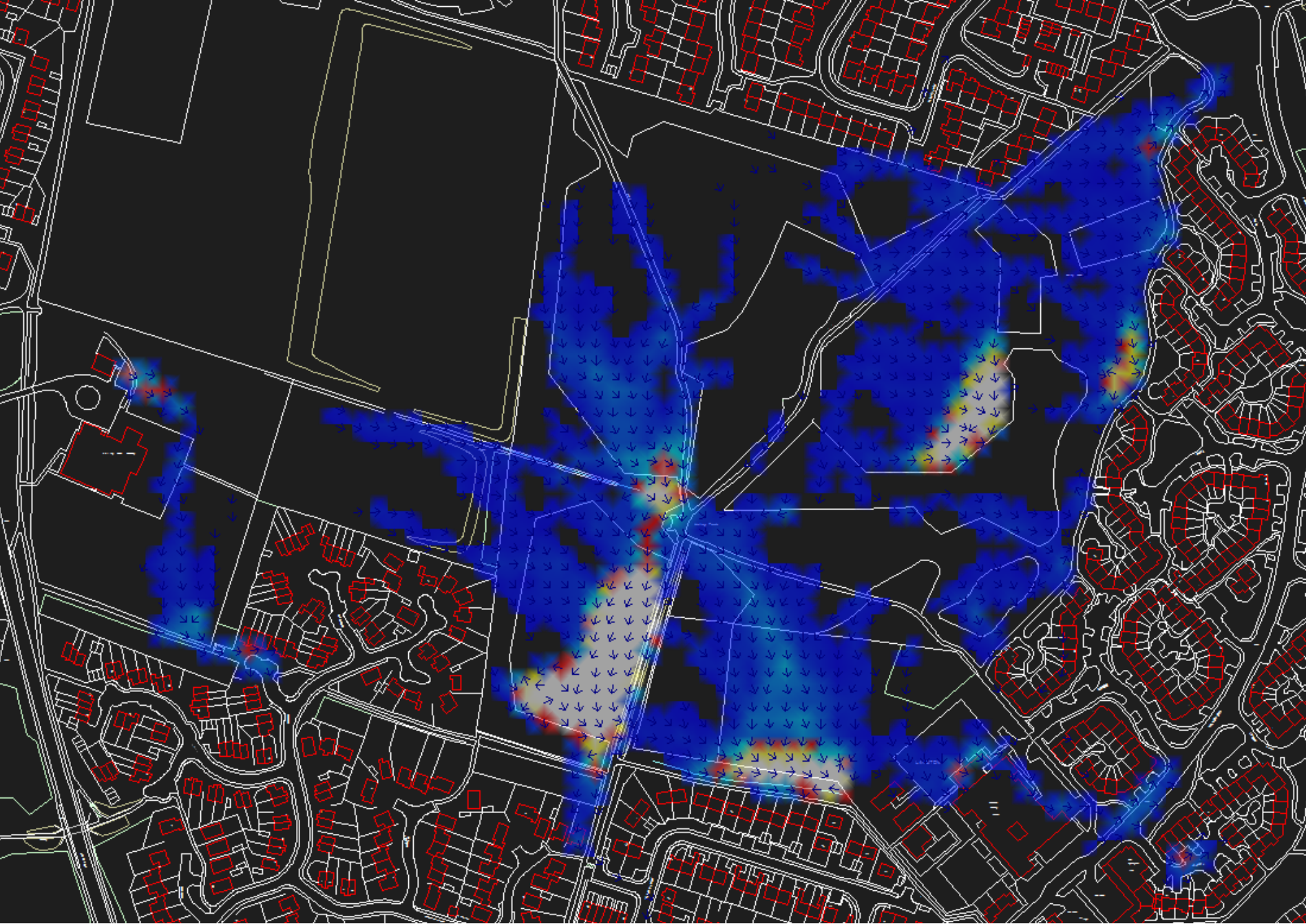
Flood Flow Analysis Proposed 1in75 event + 40% Climate Change
