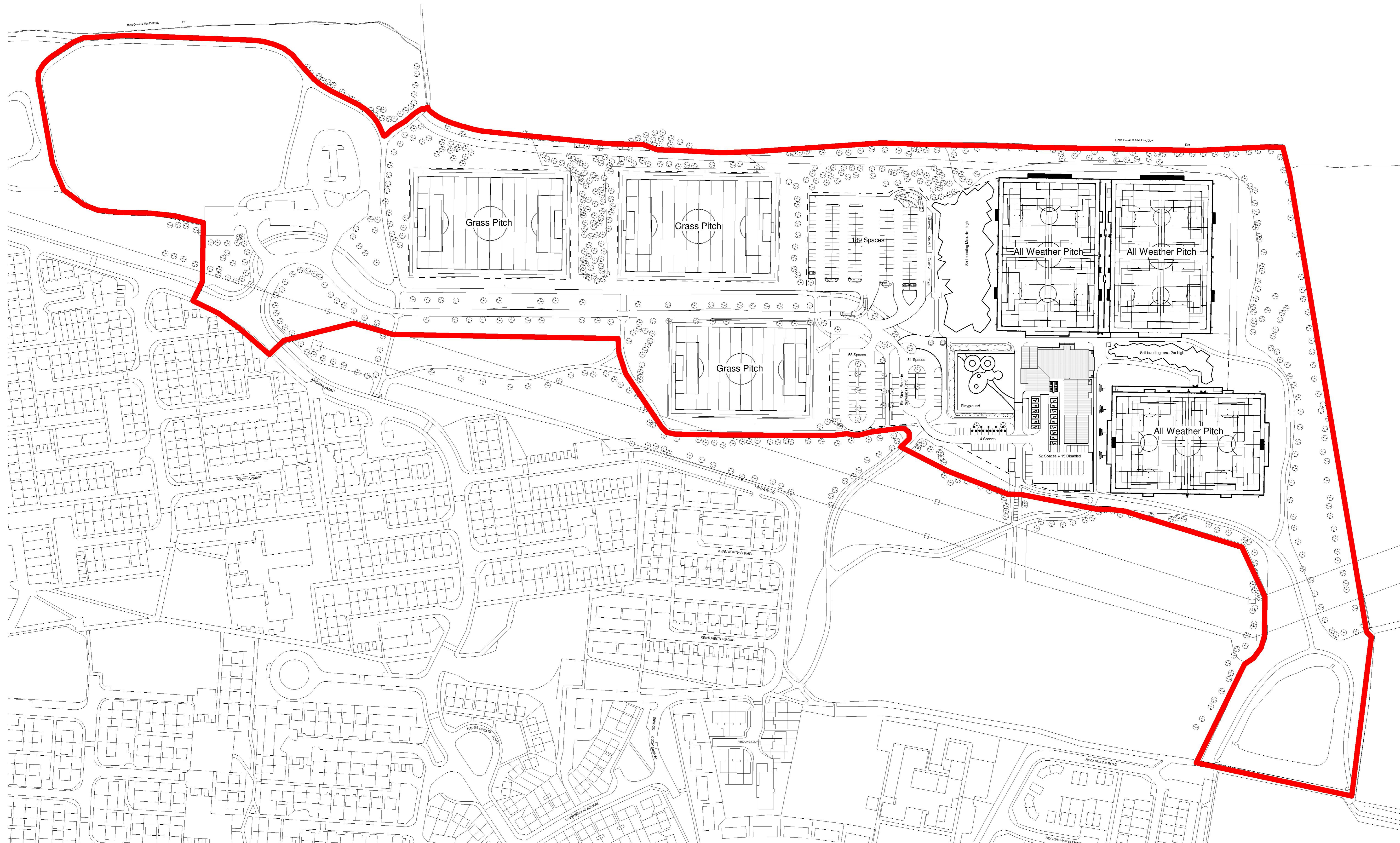
1 PROPOSED SITE PLAN (OVERALL) 1 : 1250
