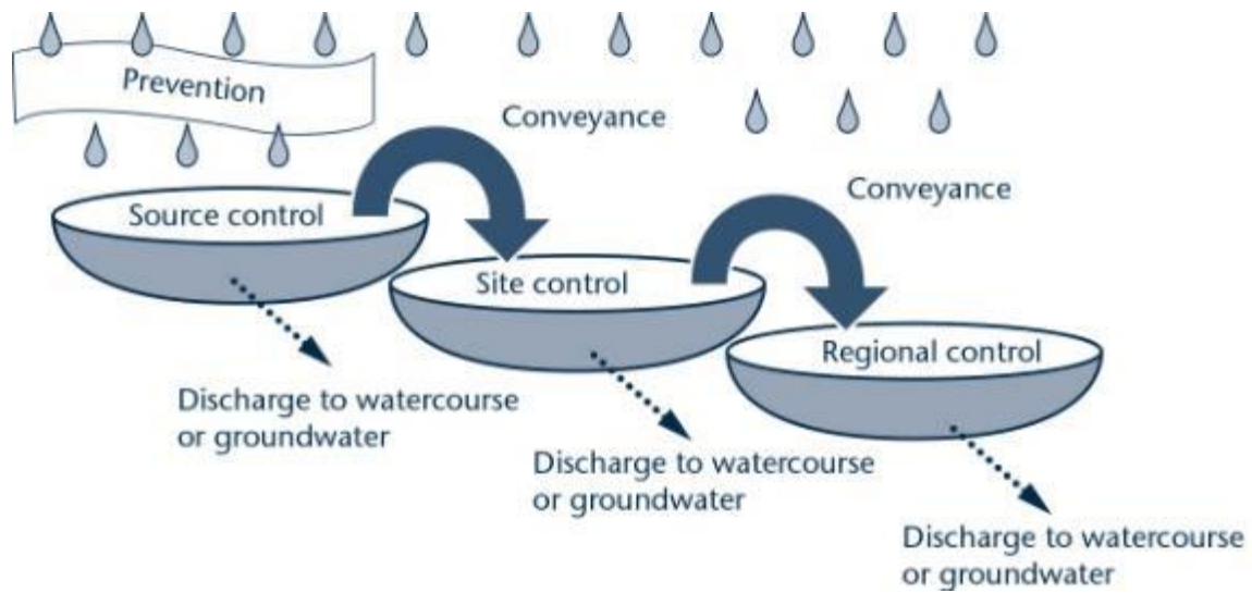
Figure 6-4 SuDS Management Train Principle 28
